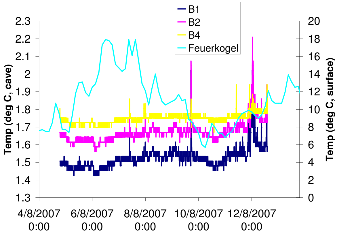
Figure 16: Temperature in Crowning Glory area with surface temperatures from Feuerkogel.
