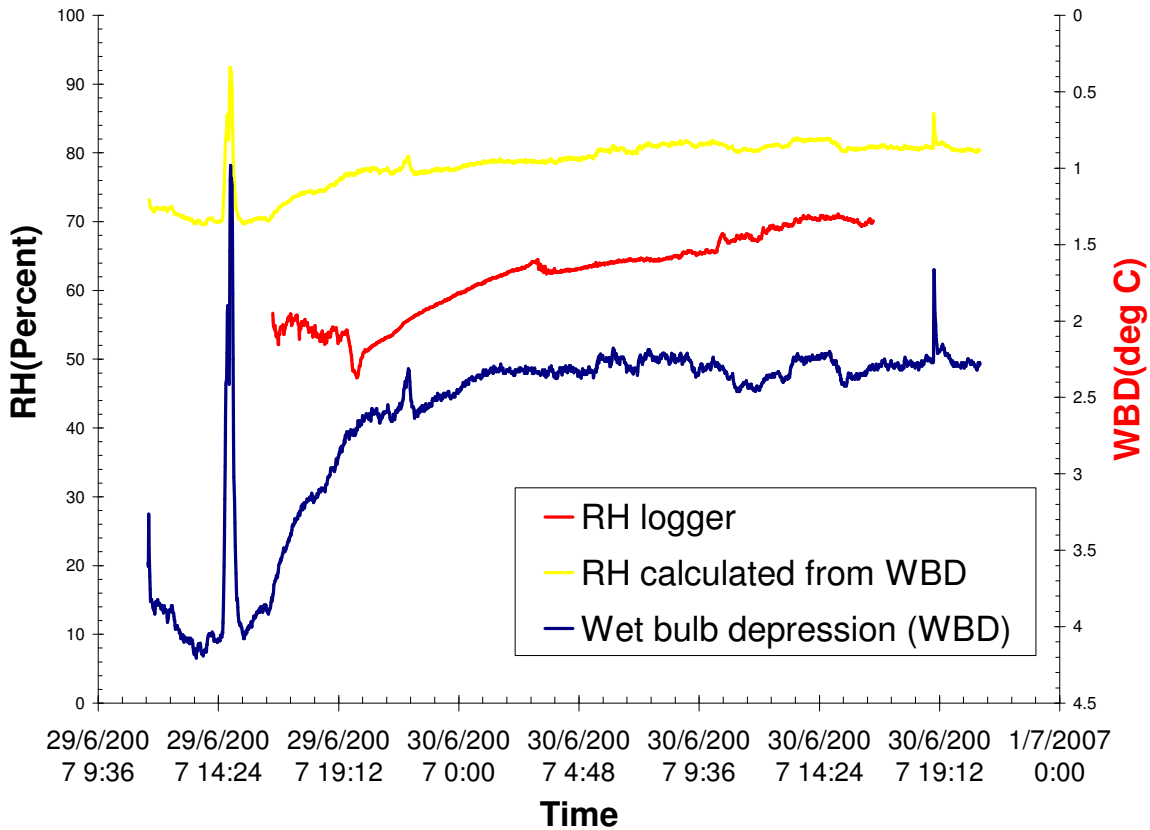
Figure 5: Testing / calibration of wet / dry bulb pairs with conventional RH sensor in CU Caving Club Tackle store
