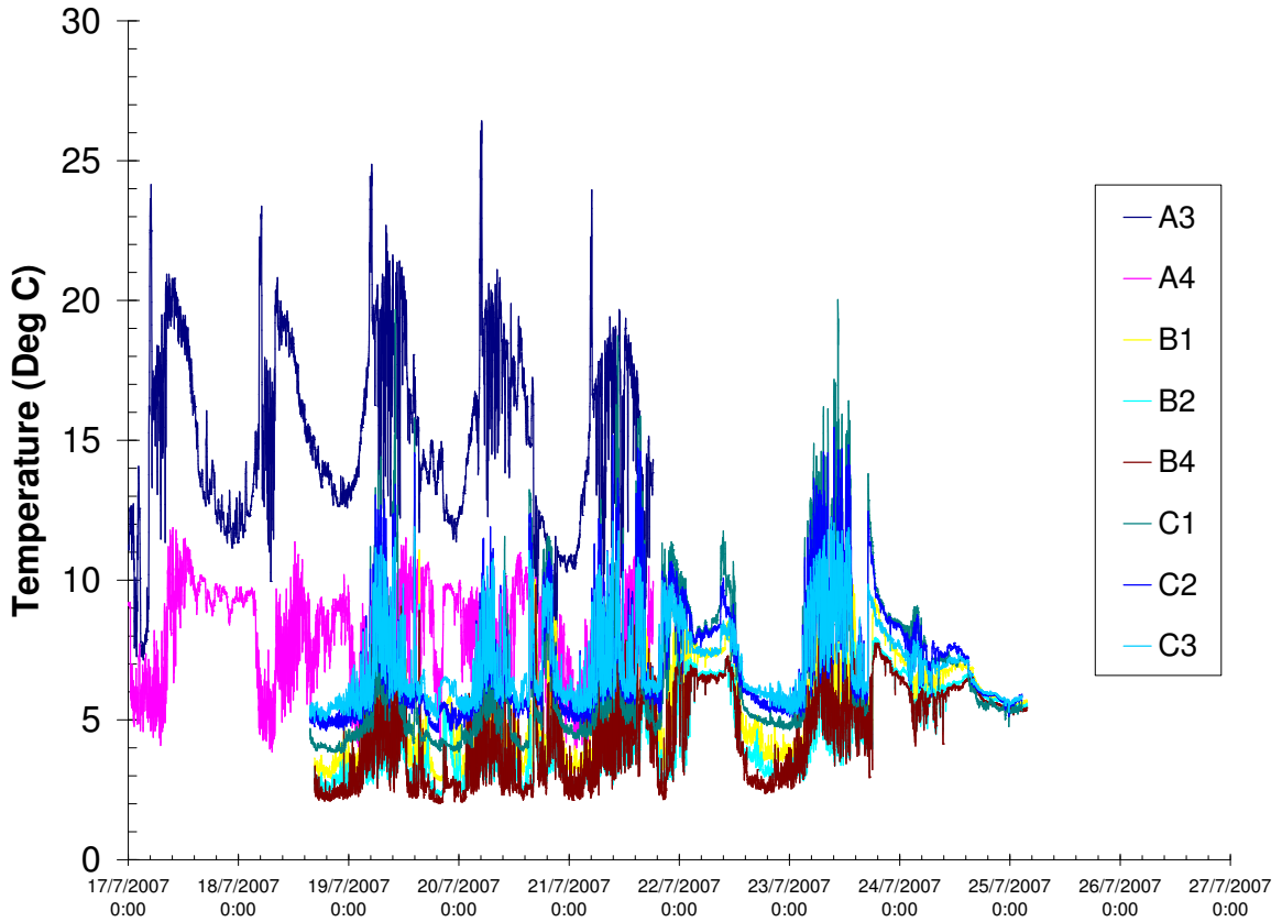
Figure 11: Temperature in Rundreisehöhle from eight thermistors. See Figure 12 for spectral analysis.
