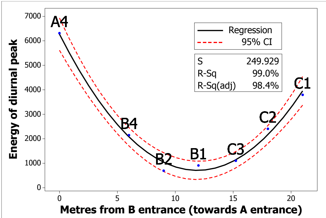
Figure 14: Amplitude of energy peak for diurnal wavelength from Fourier transform (Figure 12) for each sensor, with distance into the cave. A parabolic regression, with the equation amplitude = 6273 - 934.8m into cave + 39.26m into cave 2 fits well. Entrances are at 0 and 25m.
