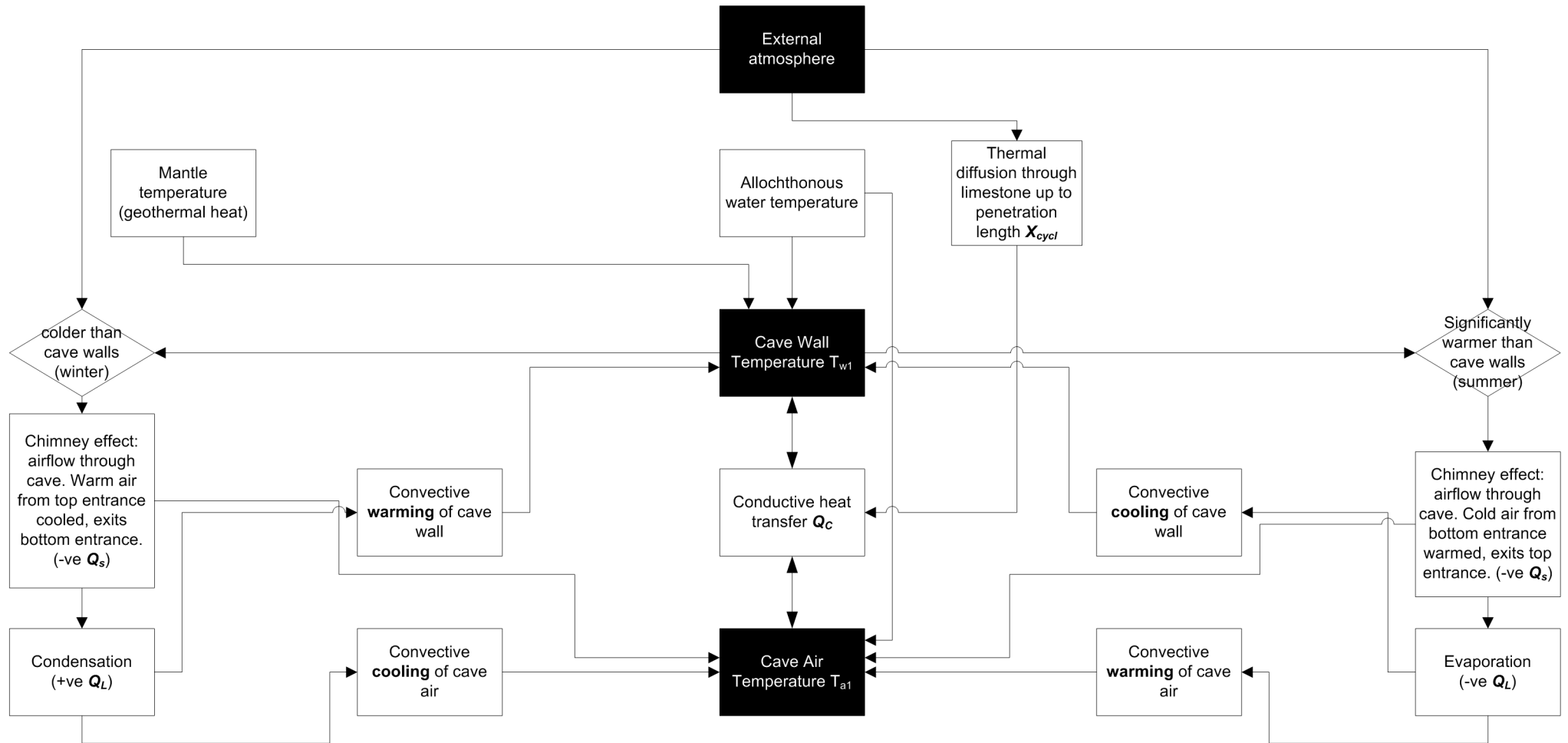
Figure 1: Schematic overview of major processes acting in cave microclimates
